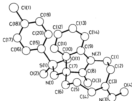
Fig. 4. The molecular structure of compound (IV).
